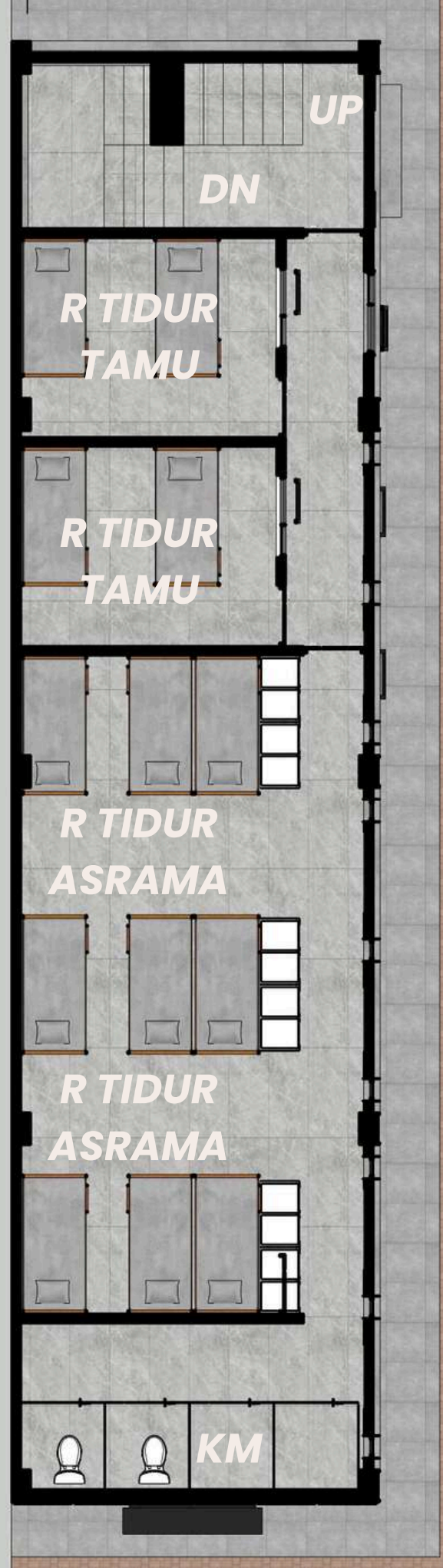
DENAH LANTAI 3
